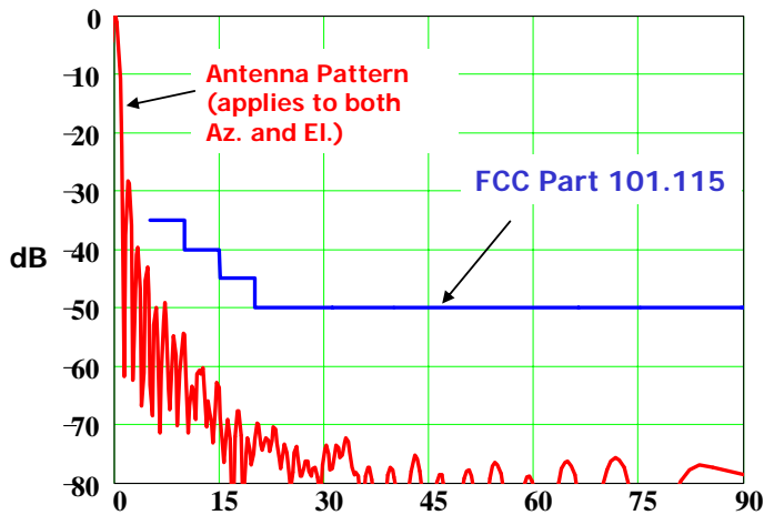
Sidelobe Pattern (71 GHz)
